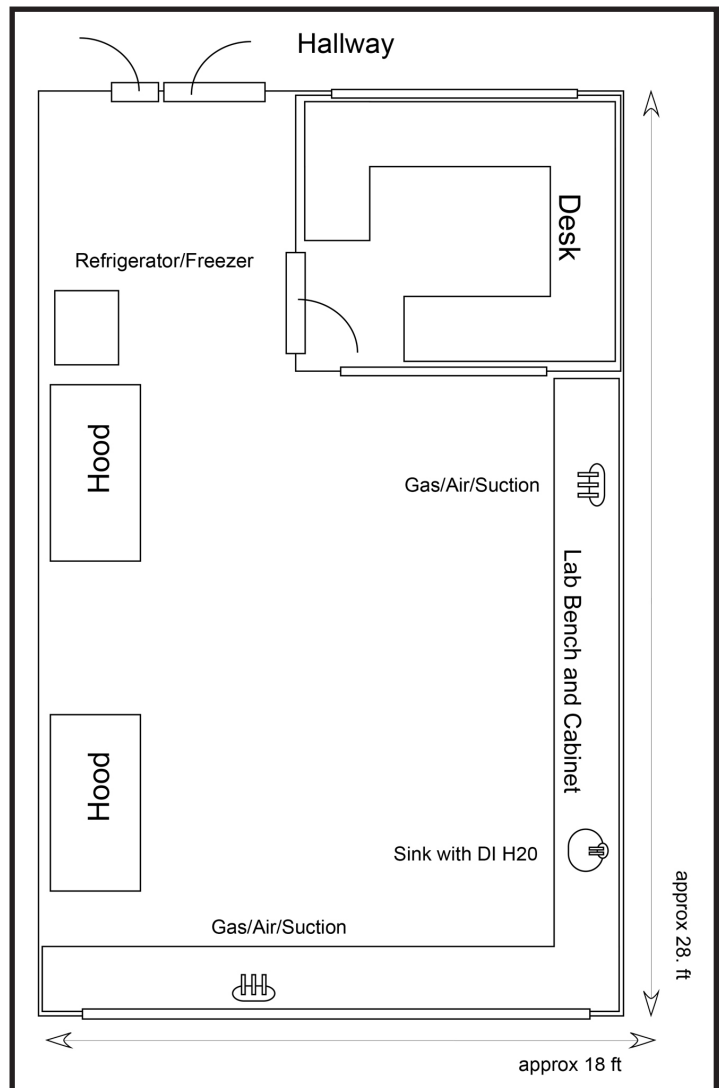
Example floor plan of a large lab.
